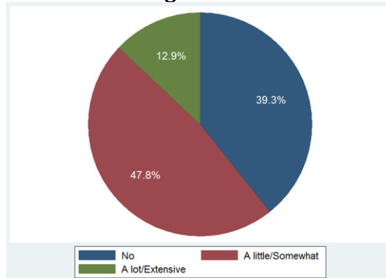
Figure 7. Have you noticed a decline in student academic performance that may be related to concerns about immigration issues?
